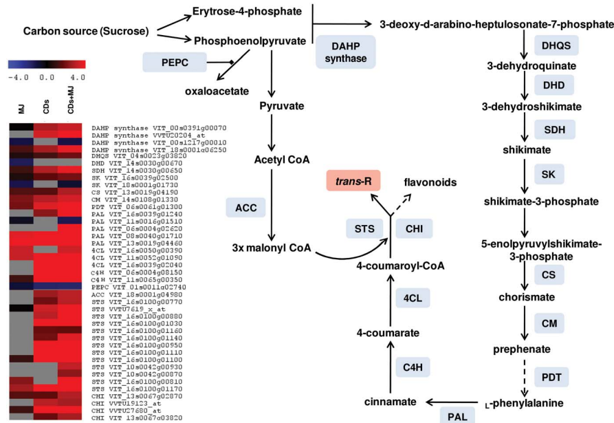
Figure 5. Modulation of trans -resveratrol biosynthesis pathway encoding enzymes gene expression by CD (cyclodextrins) and/or MJ (methyl jasmonate). Enzyme abbreviations: 4CL, 4-coumarate CoA ligase; ACC, acetyl-CoA carboxylase; C4H, cinnamate-4-hydroxylase; CHI, chalcone isomerase; CM, chorismate mutase; CS, chorismate synthase; DAHP synthase, 3-deoxy-D-arabino-heptulosonate 7-phosphate synthase; DHD, dehydroquininate dehydratase; DHQS, 3-dehydroquininate synthase; PAL, phenylalanine ammonia lyase; PDT, prephenate dehydratase; PEPC, phosphoenolpyruvate carboxylase; SDH, shikimate dehydrogenase; SK, shikimate kinase; STS, stilbene synthase. doi:10.1371/journal.pone.0109777.g005
