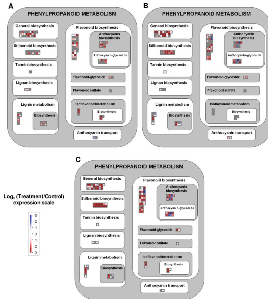
Figure 4. Mapman visualization of the significant genes in the 'Phenylpropanoid metabolism' pathway. A, MJ (methyl jasmonate); B, CD (cyclodextrins); C, CDMJ (cyclodextrins and methyl jasmonate). Resultant transcripts were considered after the average of significant redundant probesets expression values. Significant probesets according to a 5% FDR and P -value < 0.05 for model variable in the corresponding control versus treatment 24 h series maSigPro comparison. Expression changes in the treatment normalized to these in the control are shown. Red, treatment up-regulated transcripts; blue, treatment down-regulated transcripts; grey, transcripts not significant in the treatment. doi:10.1371/journal.pone.0109777.g004
