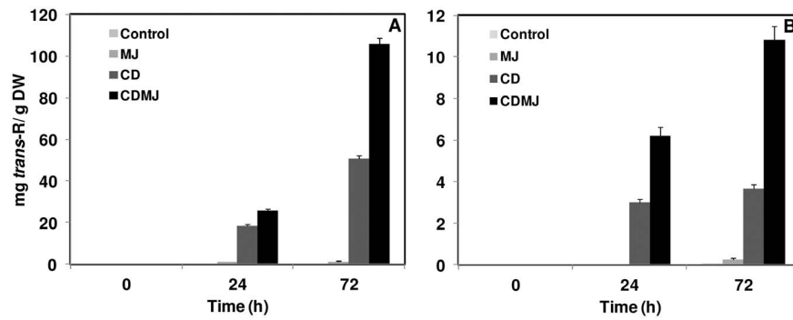
Figure 1. Effect of elicitation time course on trans -R ( trans -resveratrol) production in grapevine cells treated with CD (cyclodextrins) and/or MJ (methyl jasmonate). (A) trans -R content in the extracellular medium. (B) trans -R content in the cells. Experiments were repeated three times. Data are the mean \pm SD of the replicates.
