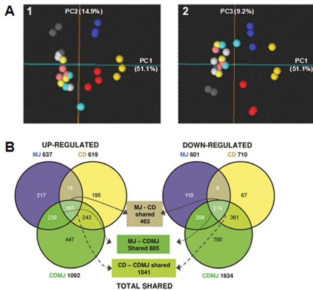
Figure 2. A, PCA over the expression dataset after the average of the redundant probesets expression values. 1, PC1 vs PC2; 2, PC1 vs PC3. Grey, Control; Blue, MJ (methyl jasmonate); Red, CD (cyclodextrins); Yellow, CD and MJ (cyclodextrins and methyl jasmonate); Light colors, just before cell treatments; Dark colors, 24 h cell treatments. B, Genes significantly regulated by elicitor treatments. C, control; MJ, methyl jasmonate; CD, cyclodextrins; CDMJ, cyclodextrins and methyl jasmonate. Venn diagram summary of significantly regulated transcripts. Non-redundant significant transcripts were obtained from probesets showing an at least 2-fold change and 5% FDR and P -value < 0.05 for model variable in the corresponding control versus treatment 24 h series maSigPro comparison. Left side, up-regulated transcripts in each treatment; Right side, down-regulated transcripts in each treatment; Center, summary of significantly regulated transcripts shared by any two treatments. doi:10.1371/journal.pone.0109777.g002
