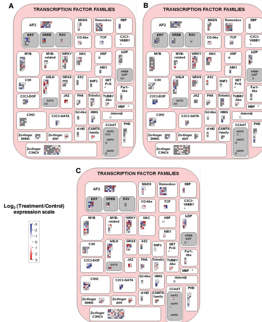
Figure 6. Mapman visualization of the significant genes in the ‘Transcription factor families’ functional category. A, MJ (methyl jasmonate); B, CD (cyclodextrins); C, CDMJ (cyclodextrins and methyl jasmonate). Resultant transcripts were considered after the average of significant redundant probesets expression values. Significant probesets according to a 5% FDR and P -value <0.05 for model variable in the corresponding control versus treatment 24 h series maSigPro comparison. Expression changes in the treatment normalized to these in the control are shown. Red, treatment up-regulated transcripts; blue, treatment down-regulated transcripts; grey, transcripts not significant in the treatment. doi:10.1371/journal.pone.0109777.g006
